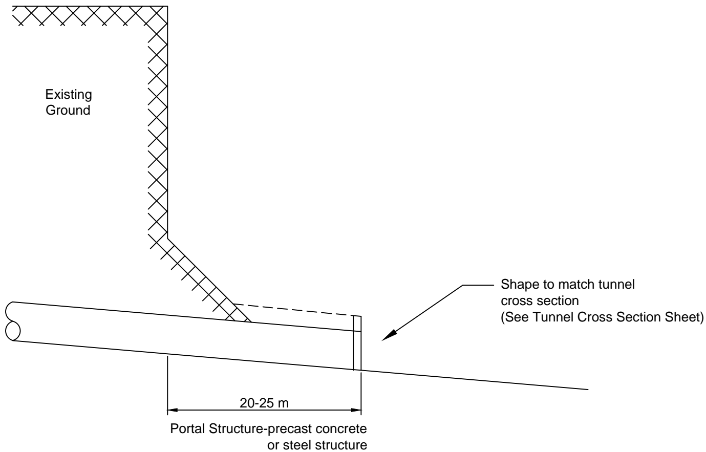
Portal at Powerhouse End (Note: Indicative only, all dimensions approximate.)
