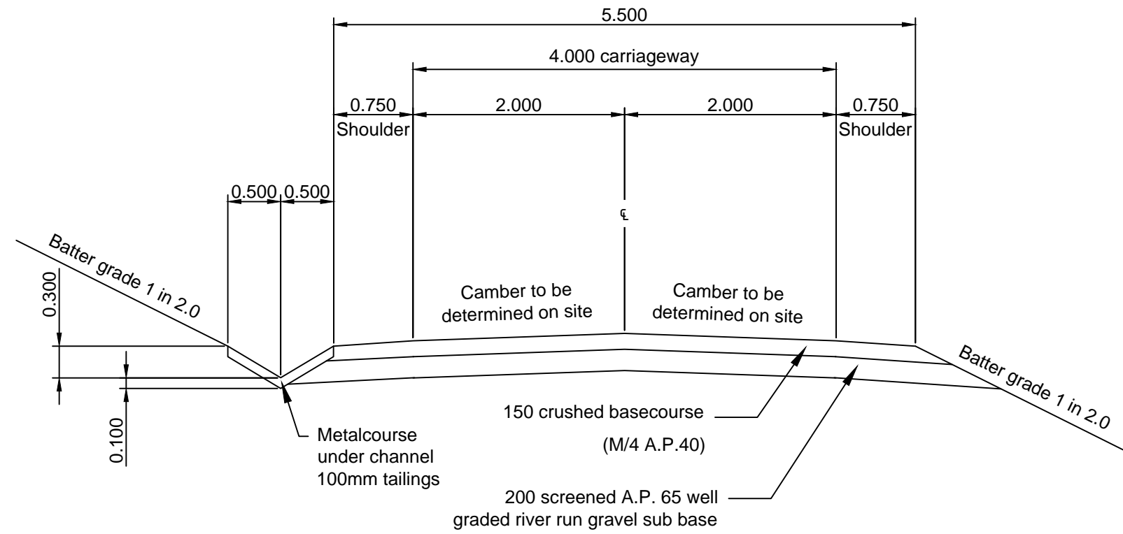
Single Lane Typical Cross Section
