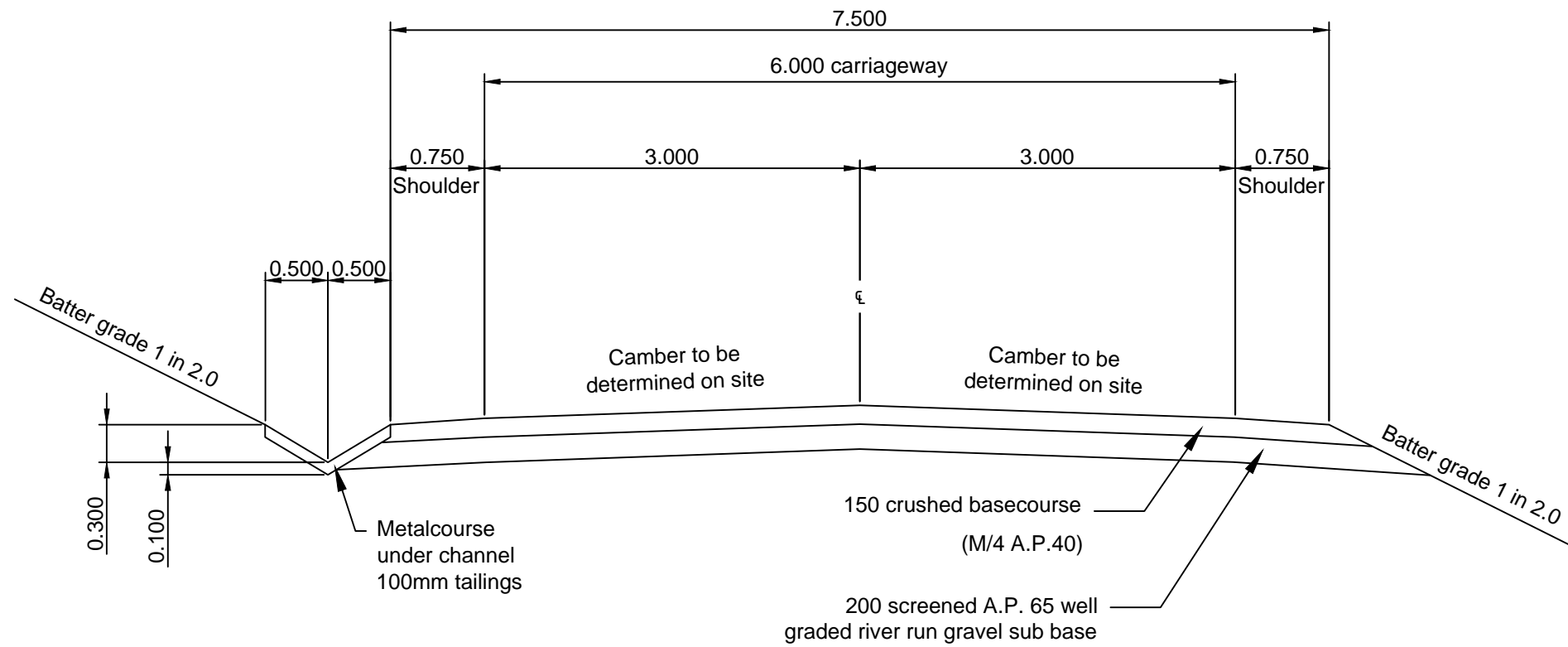
Two Lane Typical Cross Section
